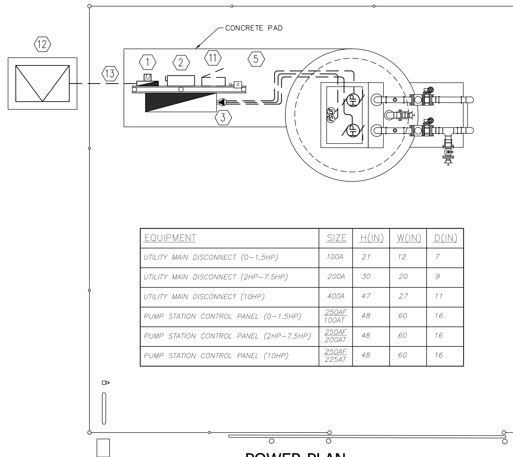
POWER PLAN
